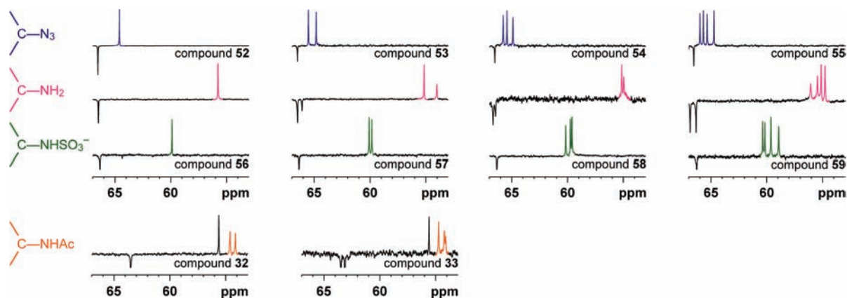
Figure 3. Comparisons of carbons attached to azido, amino, sulfonatamido, and acetamido groups in DEPT-135 spectra (solvent: \text{CD}_3\text{OD} ).
